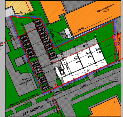
Plan parter
