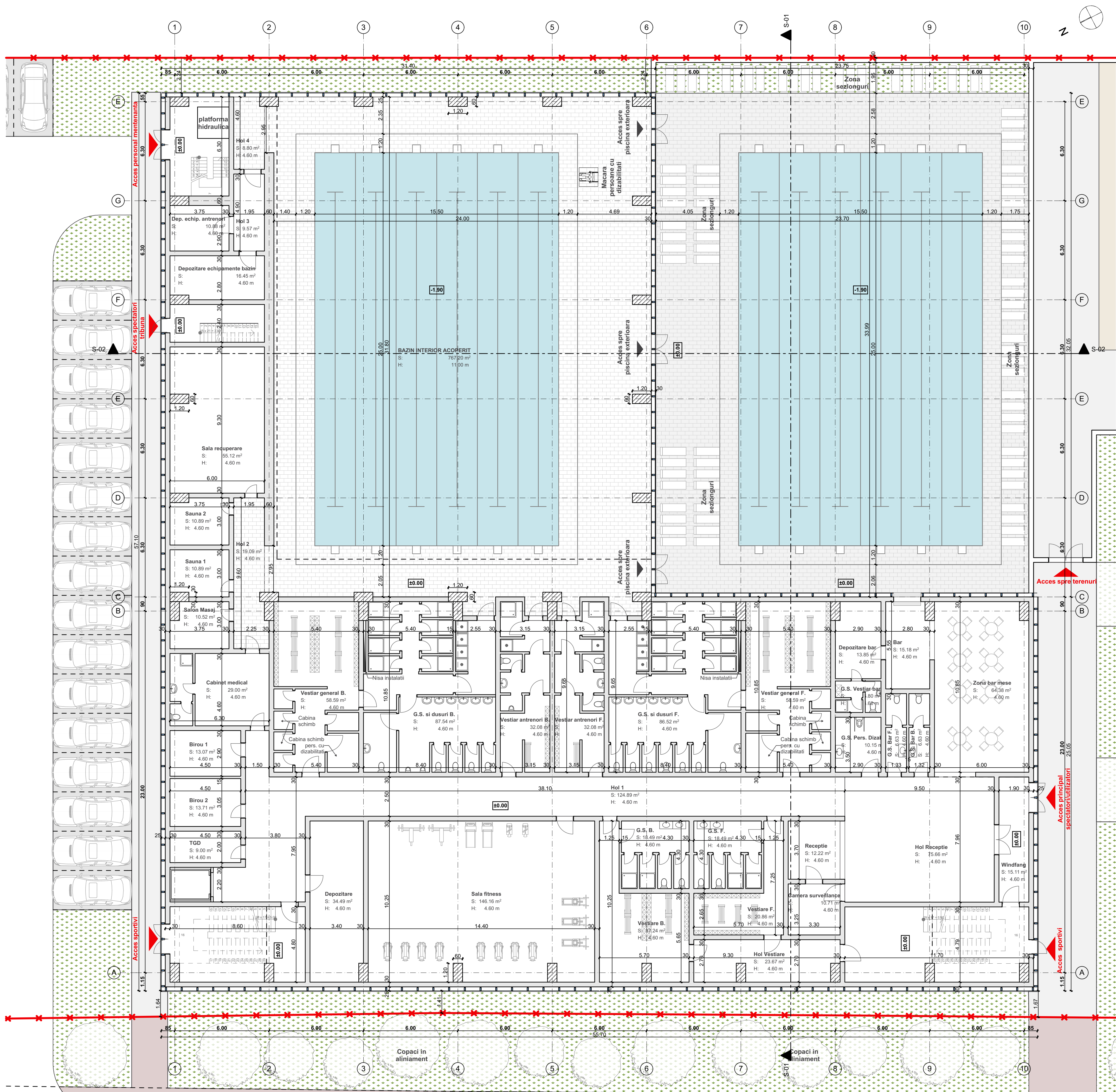
PLAN PARTER - SCARA 1:125
