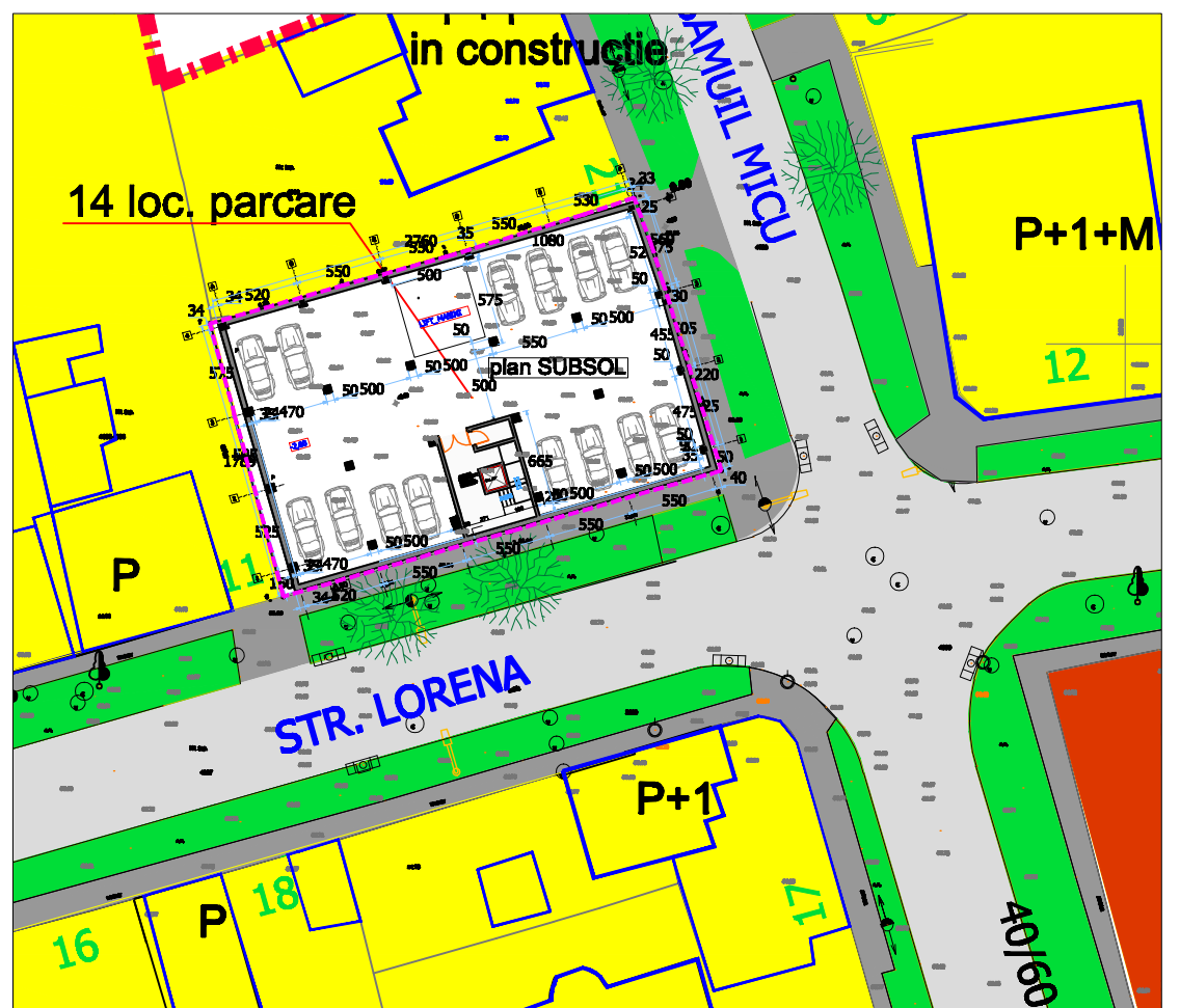
PLAN SUBSOL SC. 1:500
